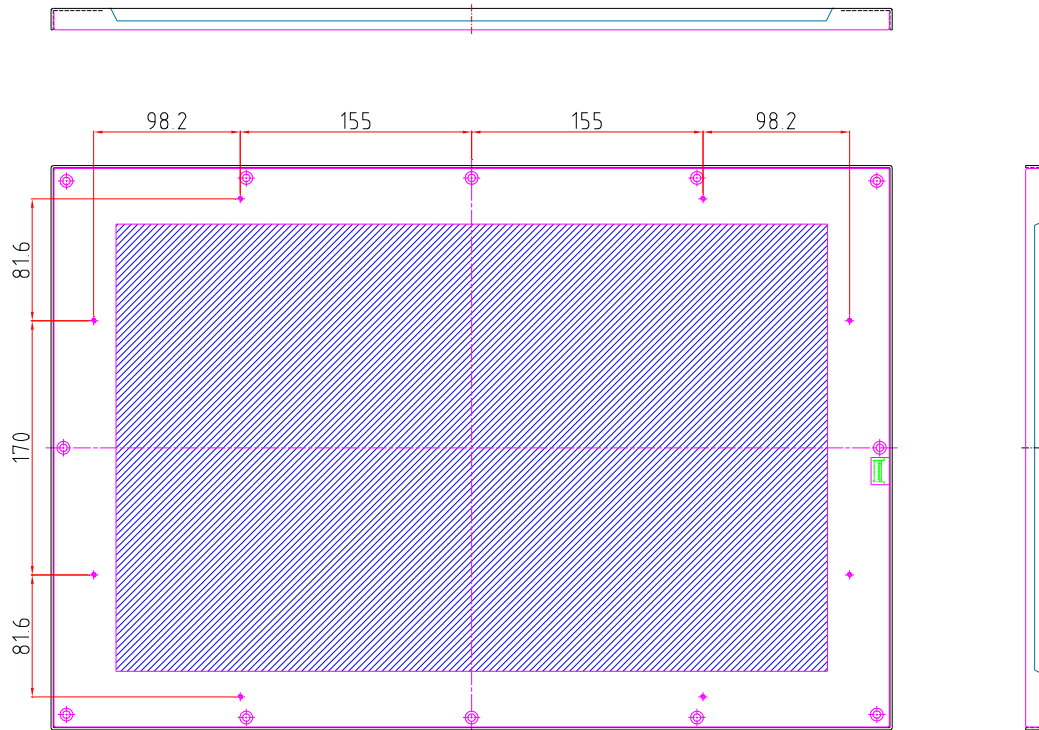
(22"IR-TOUCH : REAR-VIEW)
